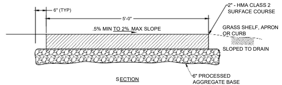
BITUMINOUS CONCRETE SIDEWALK NOT TO SCALE
