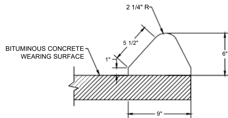
6" BITUMINOUS CONCRETE LIP CURBING NOT TO SCALE
