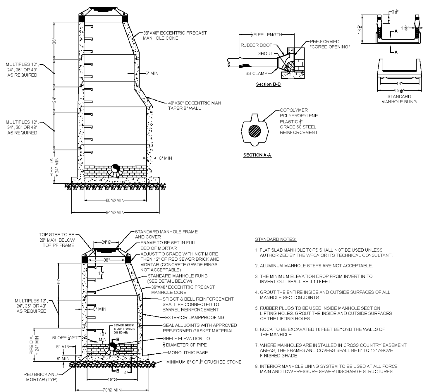
TOWN OF SIMSBURY DETAIL - STANDARD SANITARY SEWER MANHOLE NOT TO SCALE
