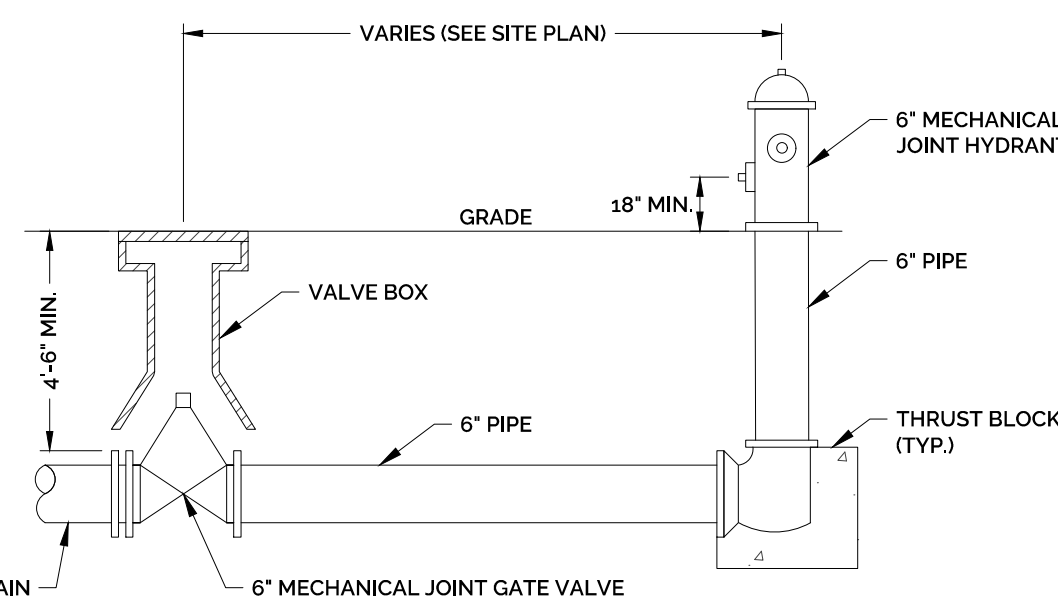
TYPICAL HYDRANT INSTALLATION NOT TO SCALE
