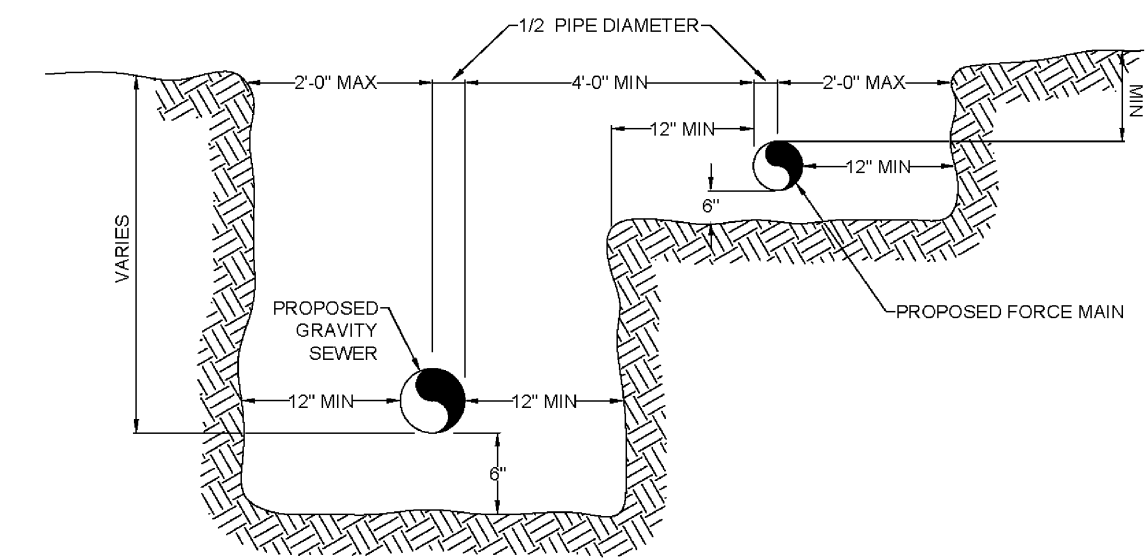
TOWN OF SIMSBURY DETAIL - COMMON GRAVITY SEWER & FORCE MAIN TRENCH NOT TO SCALE
