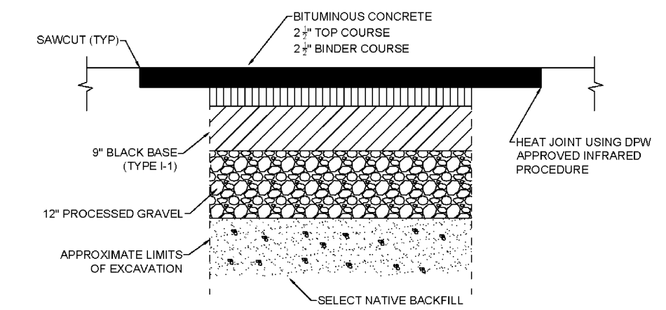
PERMANENT TRENCH REPAIR (STATE ROADS) TOWN OF SIMSBURY DETAIL - PERMANENT TRENCH REPAIR NOT TO SCALE
