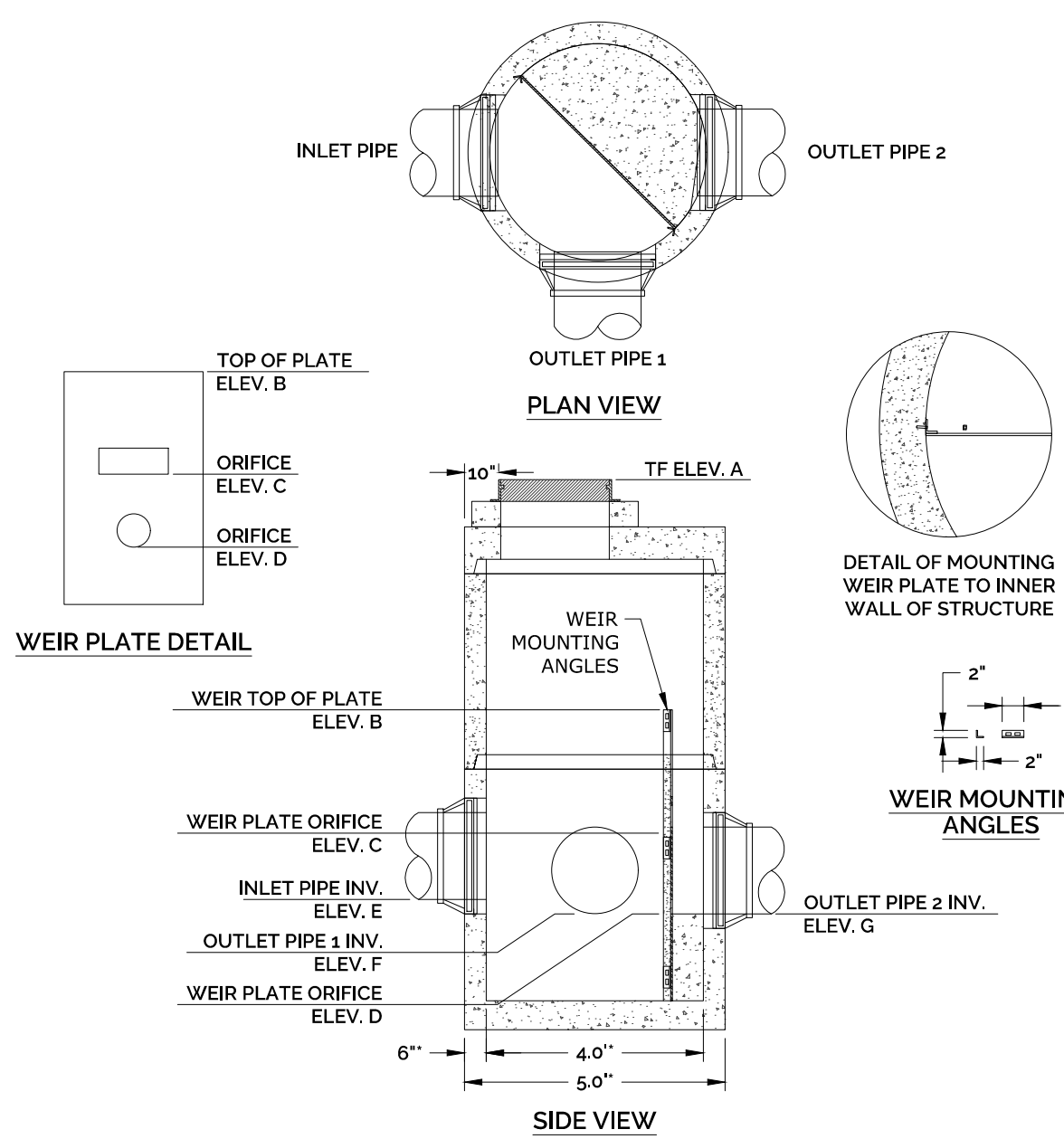
INLET/OUTLET CONTROL STRUCTURE DETAIL NOT TO SCALE
