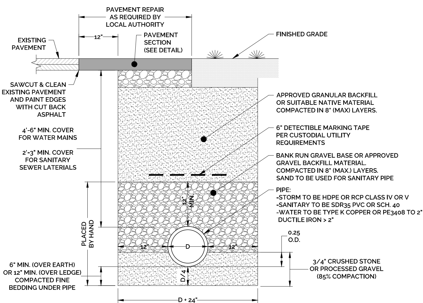
TYPICAL E/T/C UTILITY TRENCH NOT TO SCALE
