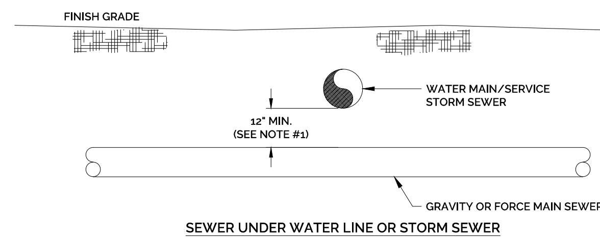
SEWER UNDER WATER LINE OR STORM SEWER
