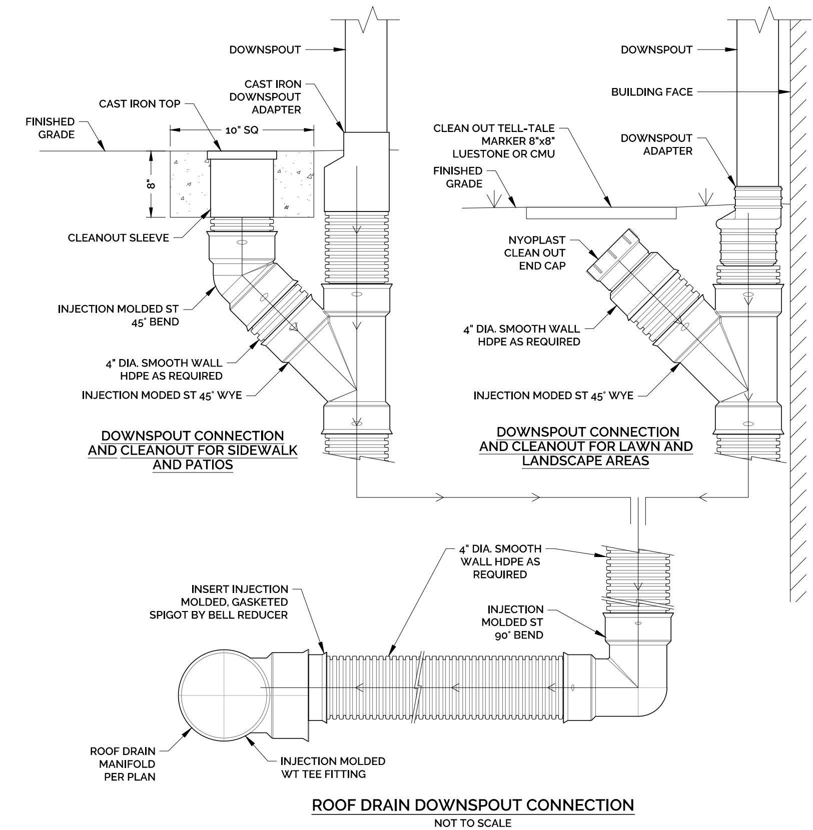
ROOF DRAIN DOWNSPOUT CONNECTION NOT TO SCALE
