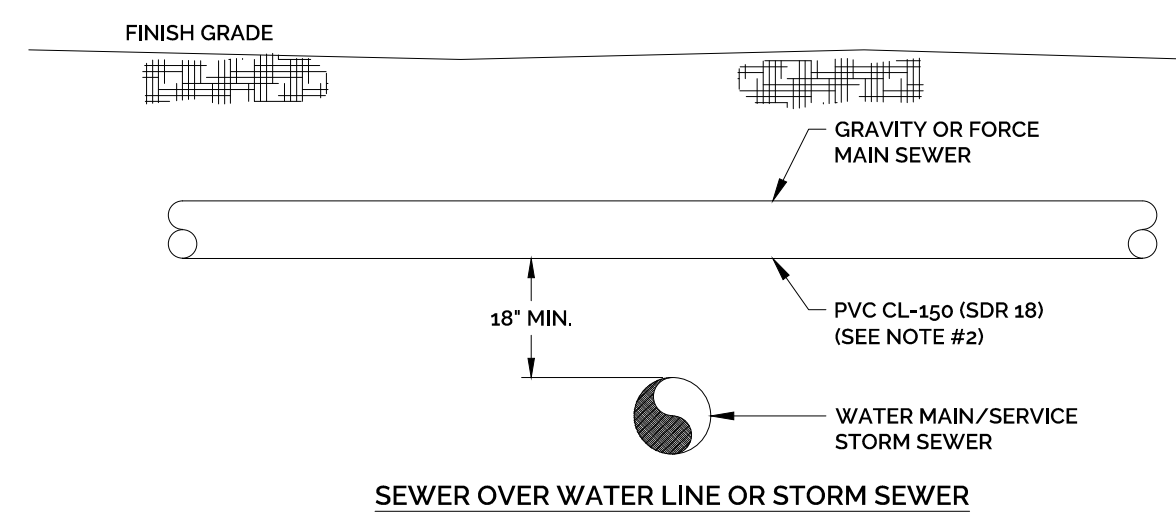
SEWER OVER WATER LINE OR STORM SEWER
