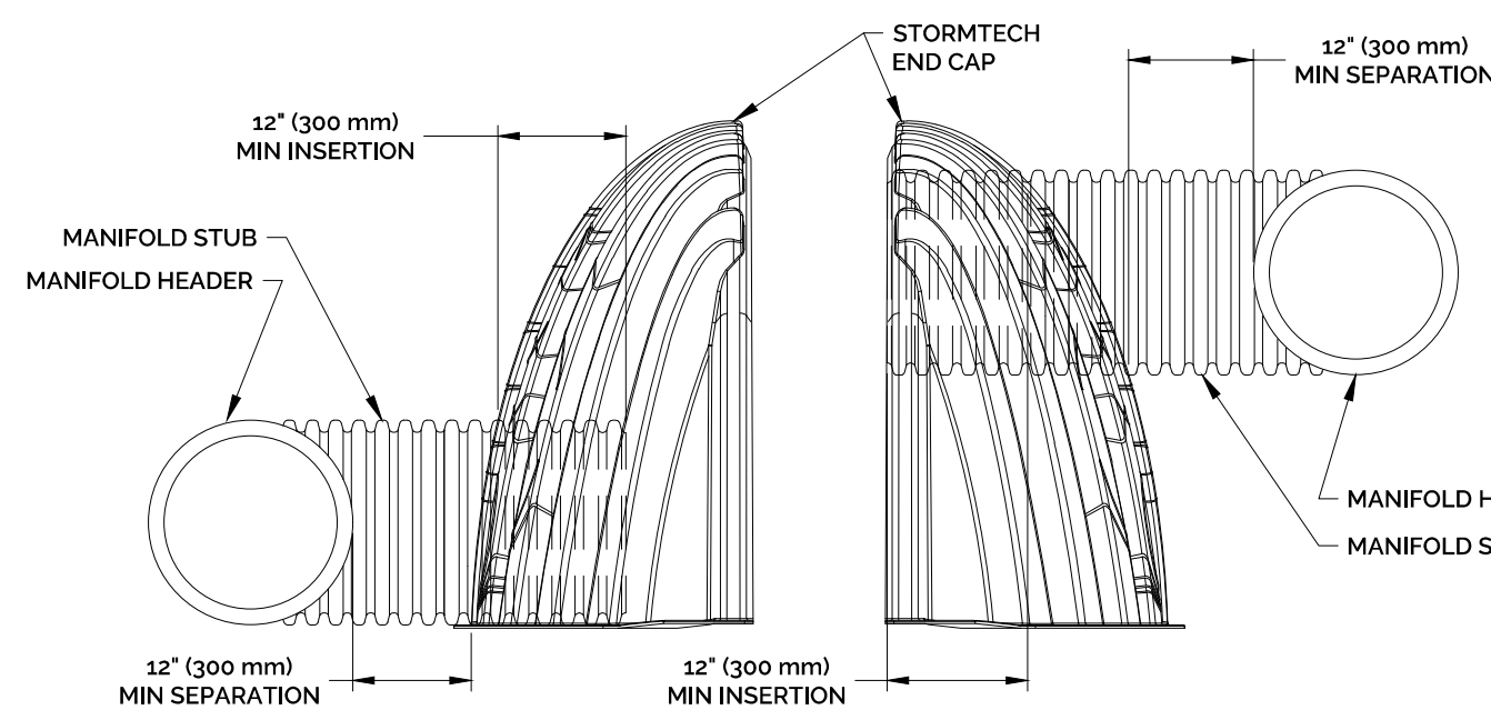
ADS STORMTECH MC-3500 END CAP INSERTION DETAIL NOT TO SCALE
