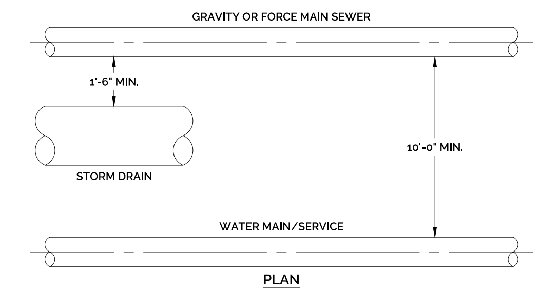
VERTICAL SEPARATION DISTANCES NOT TO SCALE
