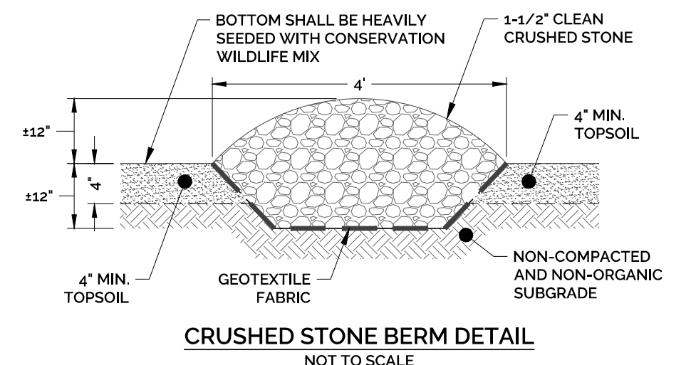
CRUSHED STONE BERM DETAIL NOT TO SCALE
