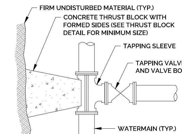
TAPPING SLEEVE & VALVE DETAIL NOT TO SCALE
