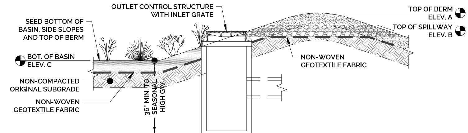
EMERGENCY SPILLWAY DETAIL NOT TO SCALE
