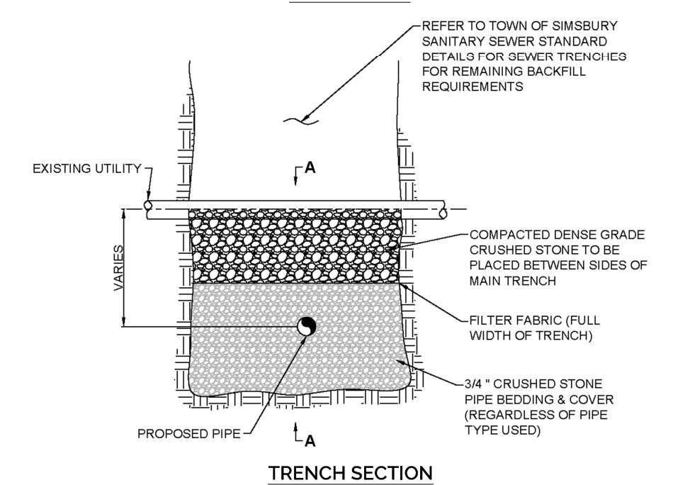
TRENCH SECTION
