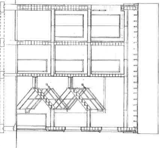
BUILDING SECTION 1/4" = 1'-0"
