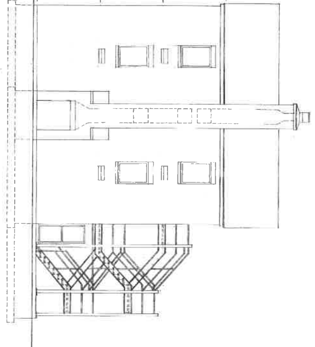
NORTH ELEVATION 1/4" = 1'-0"
