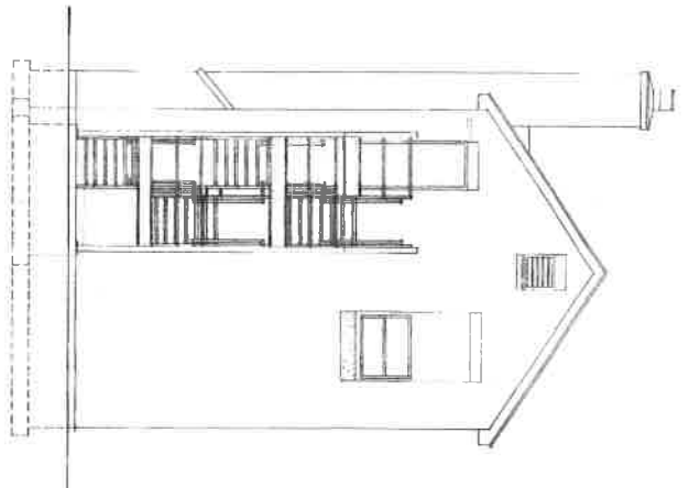
WEST ELEVATION 1/4" = 1'-0"
