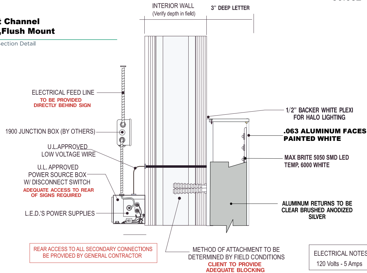
PARTIAL SECTION THRU LETTERS & INTERIOR WALL - Scale: 3" = 1'-0"
