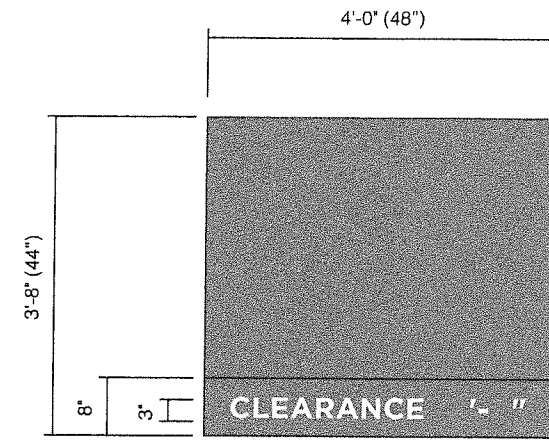
A Awning - Side View - Car Approach Side Scale: 1/2"=1'-0"
