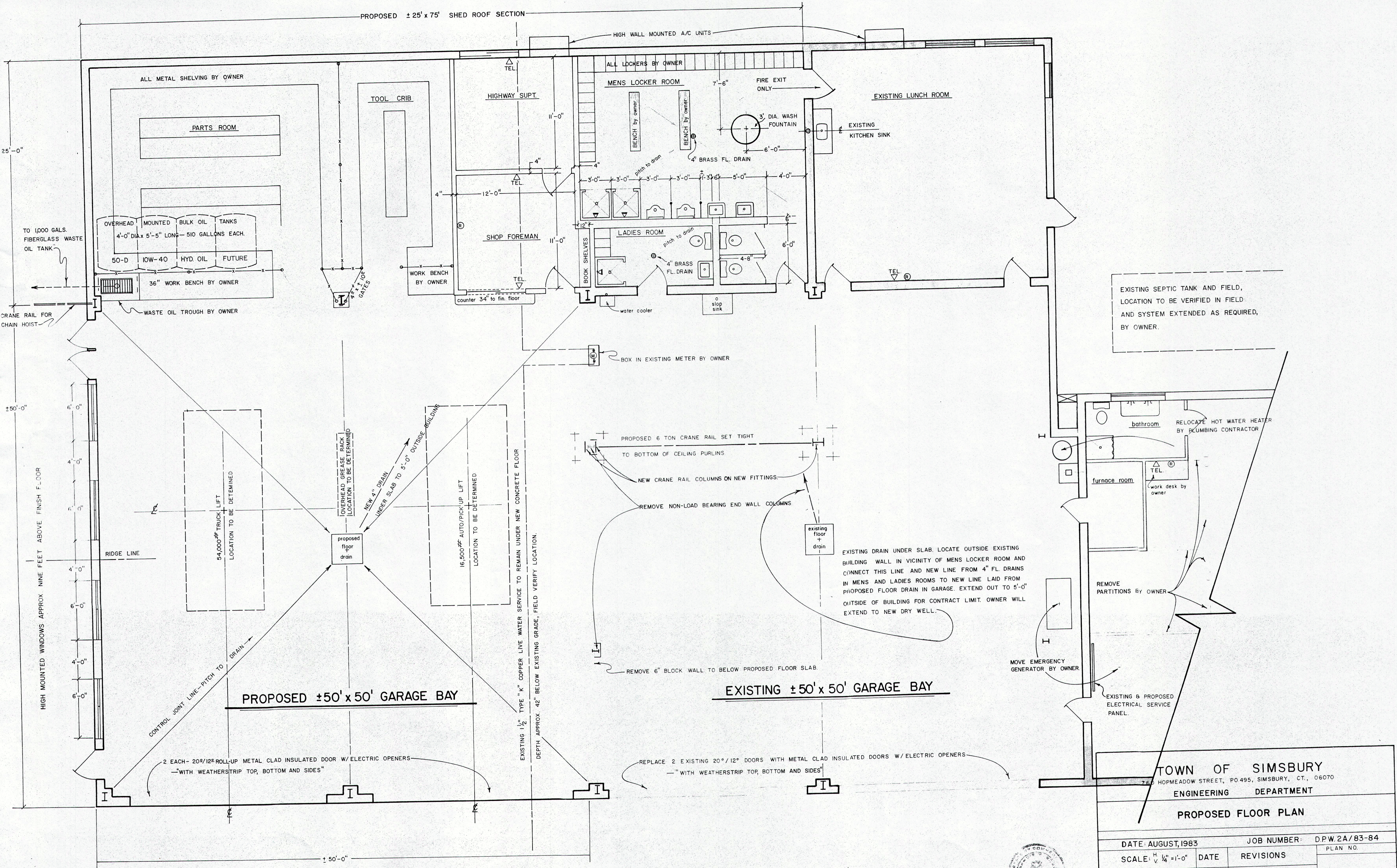
PROPOSED FLOOR PLAN SCALE: 1/4" = 1'-0"
